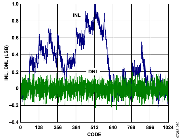
Figure 75. AUXDAC DNL and INL
