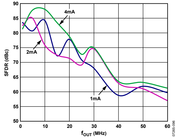
Figure 74. SFDR vs. f_{OUT}
