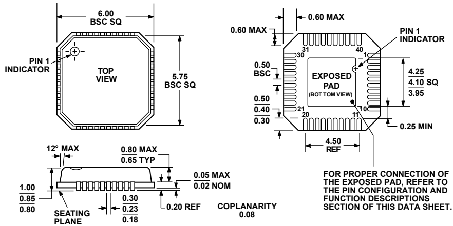
Figure 98. 40-Lead Lead Frame Chip Scale Package [LFCSP_VQ] 6 mm x 6 mm, Very Thin Quad (CP-40-1) Dimensions shown in millimeters
