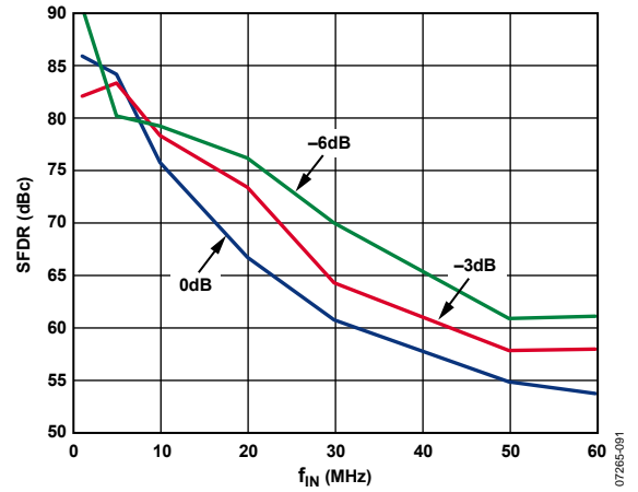
Figure 70. SFDR vs. Digital Input Level 3.3 V
